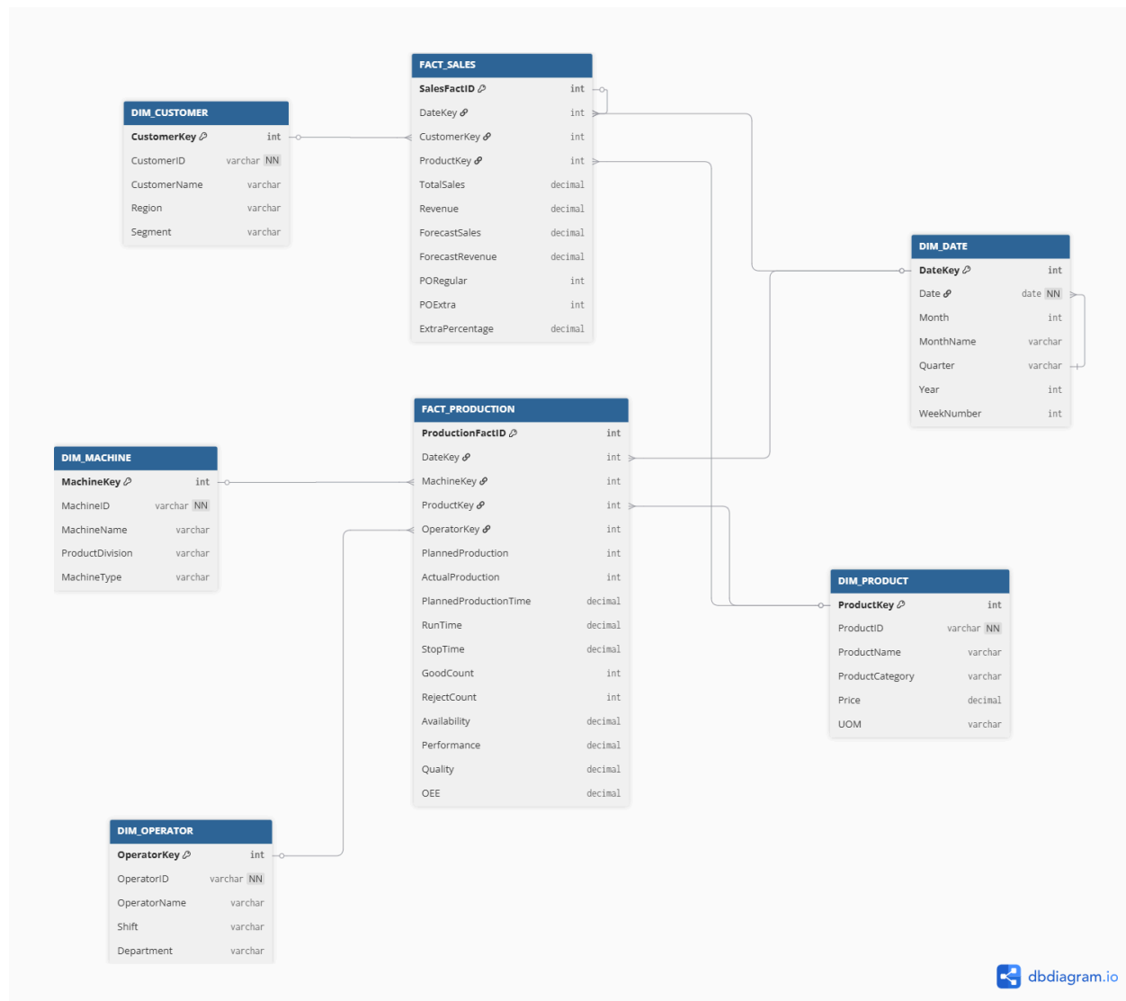
Figure 7.0 Star Schema
